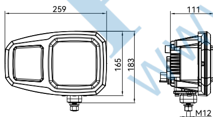
VERTICAL MOUNTING
