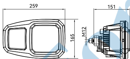
HORIZONTAL MOUNTING
