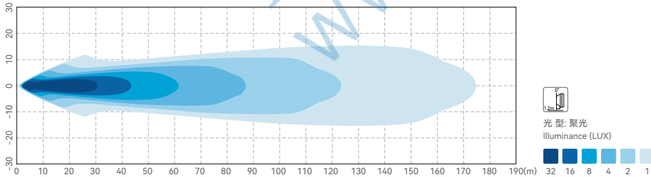
WK-64
