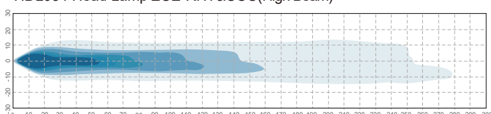
HDL034 Head Lamp ECE-RHT&CCC(High Beam)
