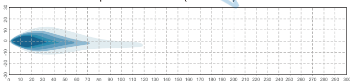
HDL034 Head Lamp ECE-RHT&CCC(Low Beam)
