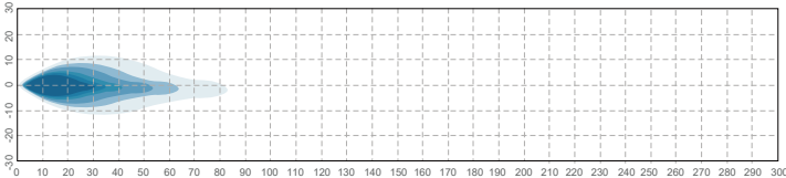
HDL034 Head Lamp Motorcycle(Low Beam)
