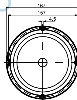
Surface Mount
